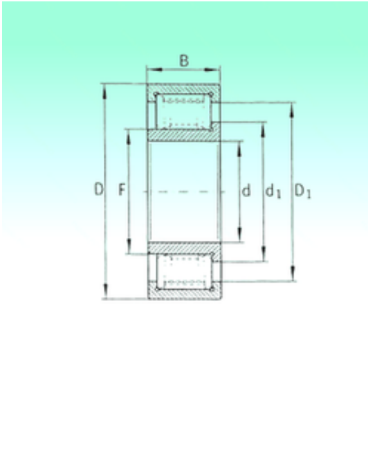
ZSL192320 Bearing 2D drawings and 3D CAD models
